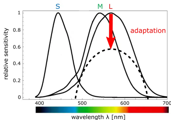
Fig. 2: Adaptation of the L cone.
